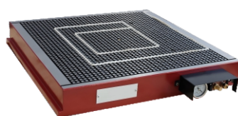
Vacuum Chuck
