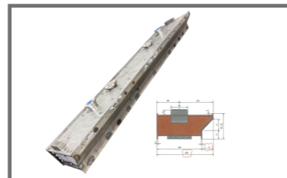
Magnetic Formwork for Robot Arm
